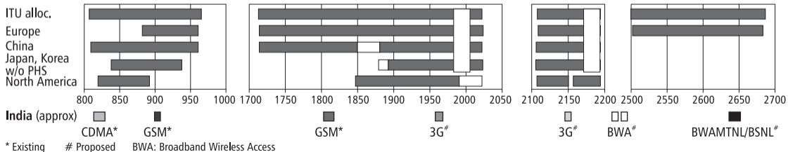
Figure 2: SPECTRUM ALLOCATED FOR 2G & 3G (Excluding satellite)
